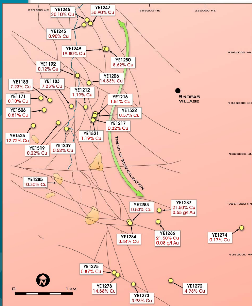
CHALCOPYRITE/BORNITE MINERALISATION KOMBRUKU PROSPECT
